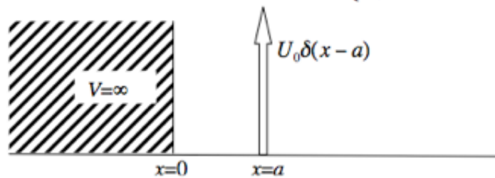
Figure 6.16: Infinite Wall + Delta Function
