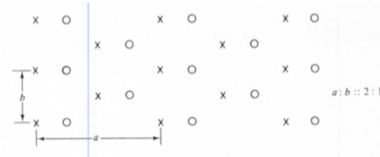
Figure 14.6: 2-Dimensional Crystal - Centered Rectangular Bravais Lattice with 2 Atoms per Primitive Unit Cell
