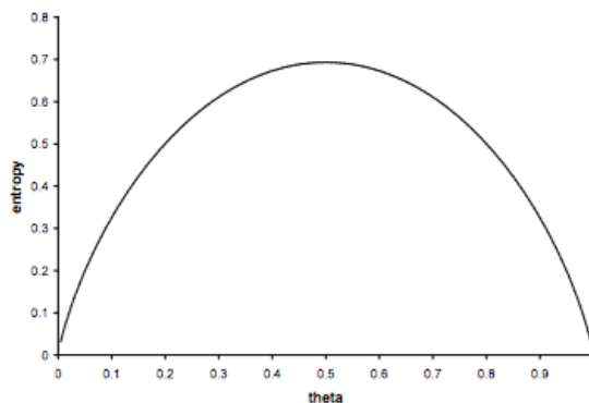
Figure 4.1: The entropy as a function of \theta
