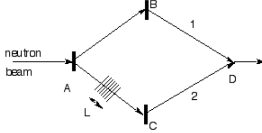
Figure 7.1: Neutron Interferometer Setup
