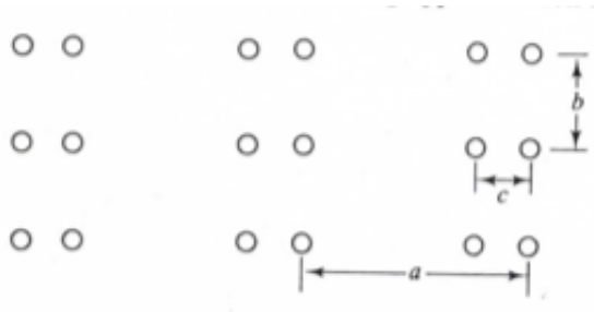
Figure 14.5: 2-Dimensional Crystal - Rectangular Bravais Lattice with 2 Atoms per Primitive Unit Cell
