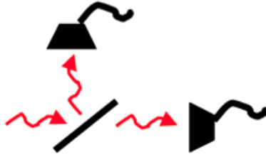
Figure 5.4: Beam Splitter
