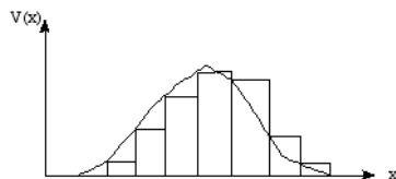
Figure 6.8: Arbitrary Barrier Potential
