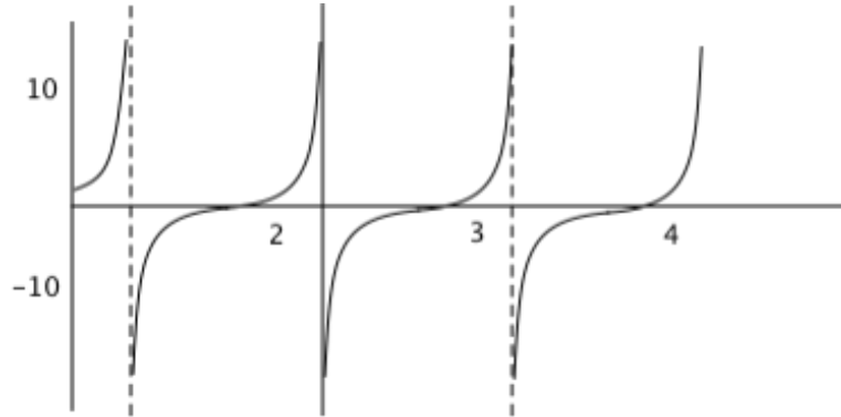
Figure 6.4: Plot of \frac{\Gamma(1/4-x)}{\Gamma(3/4-x)}
