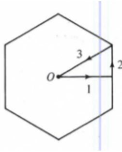
Figure 14.4: Paths in the First Brillouin Zone
