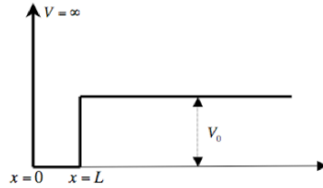
Figure 6.11: Half-Infinite, Half-Finite Well
