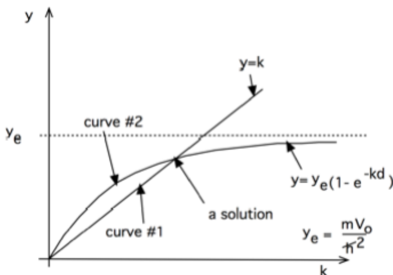
Figure 6.3: Staircase Function
