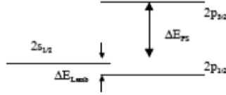
Figure 8.5: n = 2 Spectrum in Hydrogen
