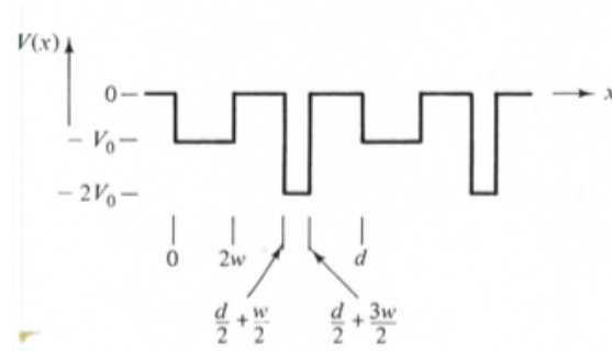
Figure 14.2: Piecewise Constant Potential - 2 Atoms per Primitive Cell
