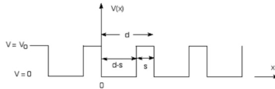
Figure 14.1: Piecewise Constant Potential - 1 Atom per Primitive Cell
