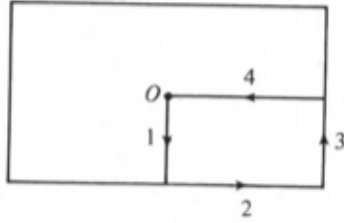
Figure 14.3: Paths in the First Brillouin Zone
